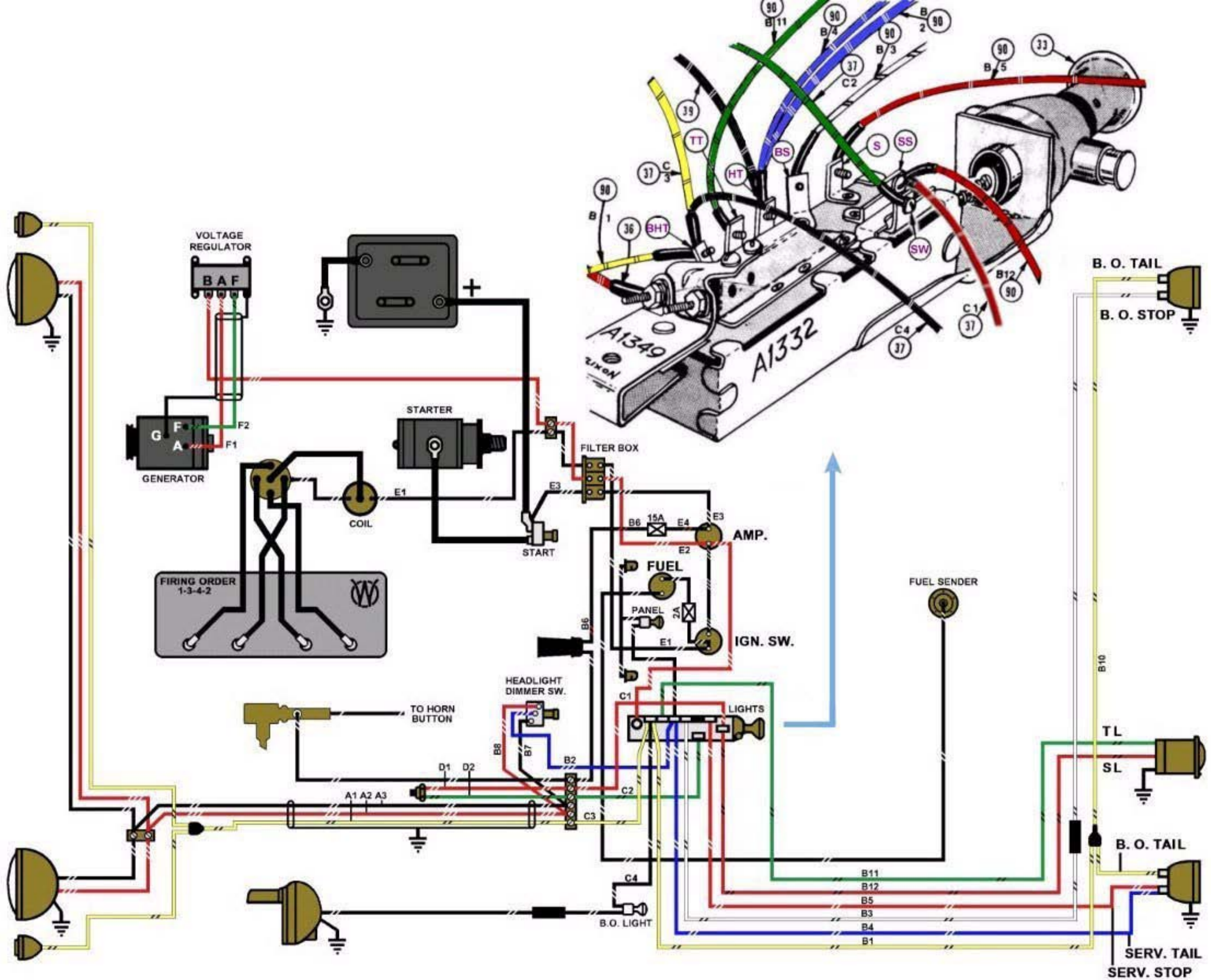
PUSH PULL SWITCH MB / GPW WIRING DIAGRAM
